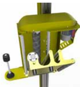
The patented easy load S-carriage offers superior pre-stretch and film tension control. It also allows extremely easy film loading.
